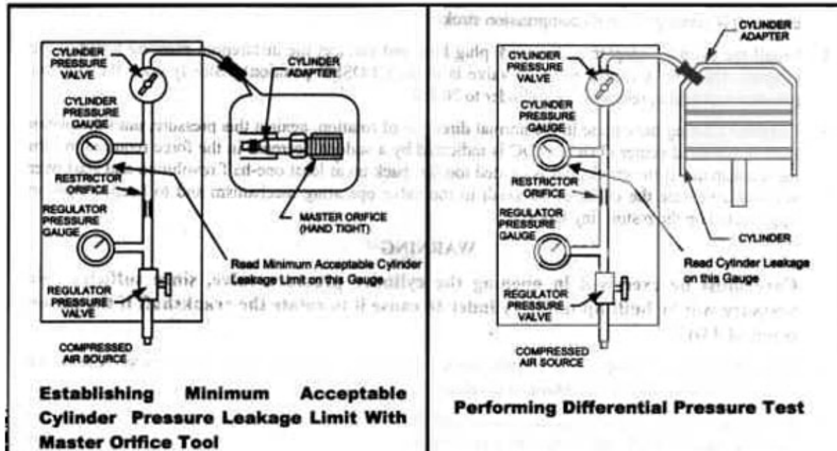
FIGURE 4 Differential Pressure Test Equipment
