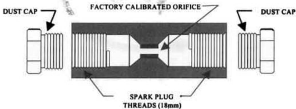
FIGURE 3 MASTER ORIFICE P/N 646953
