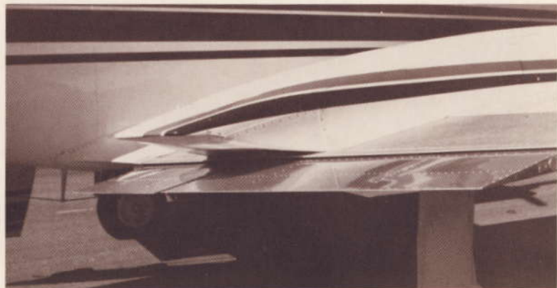
At the preselected flap takeoff position (10-degree deployment), the aft movement of the flap adds 25.3 sq. ft. of wing area.
